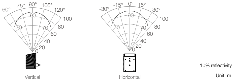
Figure 3.1.2 Effective FOV of the Mid-70
