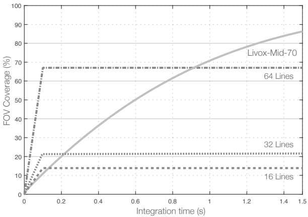
Figure 1.2.2 The FOV coverage of the Mid-70 and non-Livox LiDAR sensors using common mechanical scanning methods. The 16-line non-Livox LiDAR sensor has a vertical FOV of 30°, the 32-line non-Livox LiDAR sensor is 41°, and the 64-line non-Livox LiDAR sensor is 27°.
