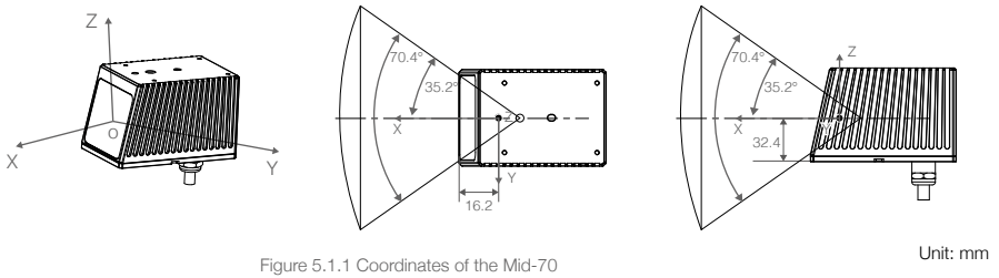
Figure 5.1.1 Coordinates of the Mid-70
