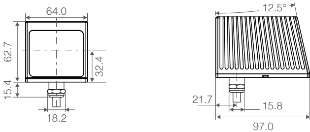
Figure 3.2.1 The Mid-70 Dimensions (refer to Appendix 1)
