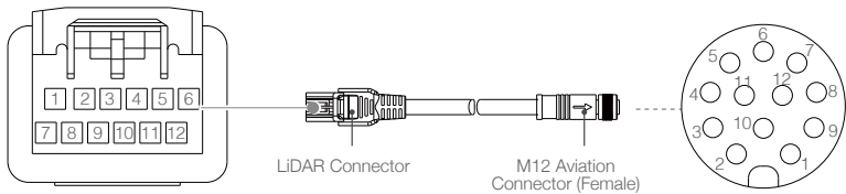
Figure 2.1.1 Conversion Cable
