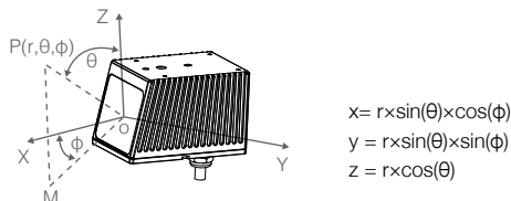
Figure 5.2.1.1 Relationship between Cartesian coordinates and Spherical coordinates
