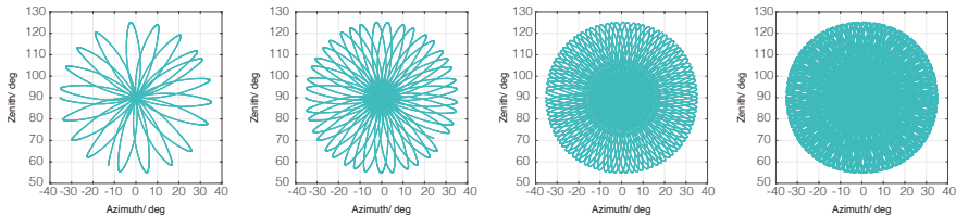
Figure 1.2.1 Point cloud patterns of the Livox Mid-70 accumulated over an extended period
