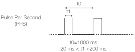
Figure 5.2.2.1 Pulse Per Second
